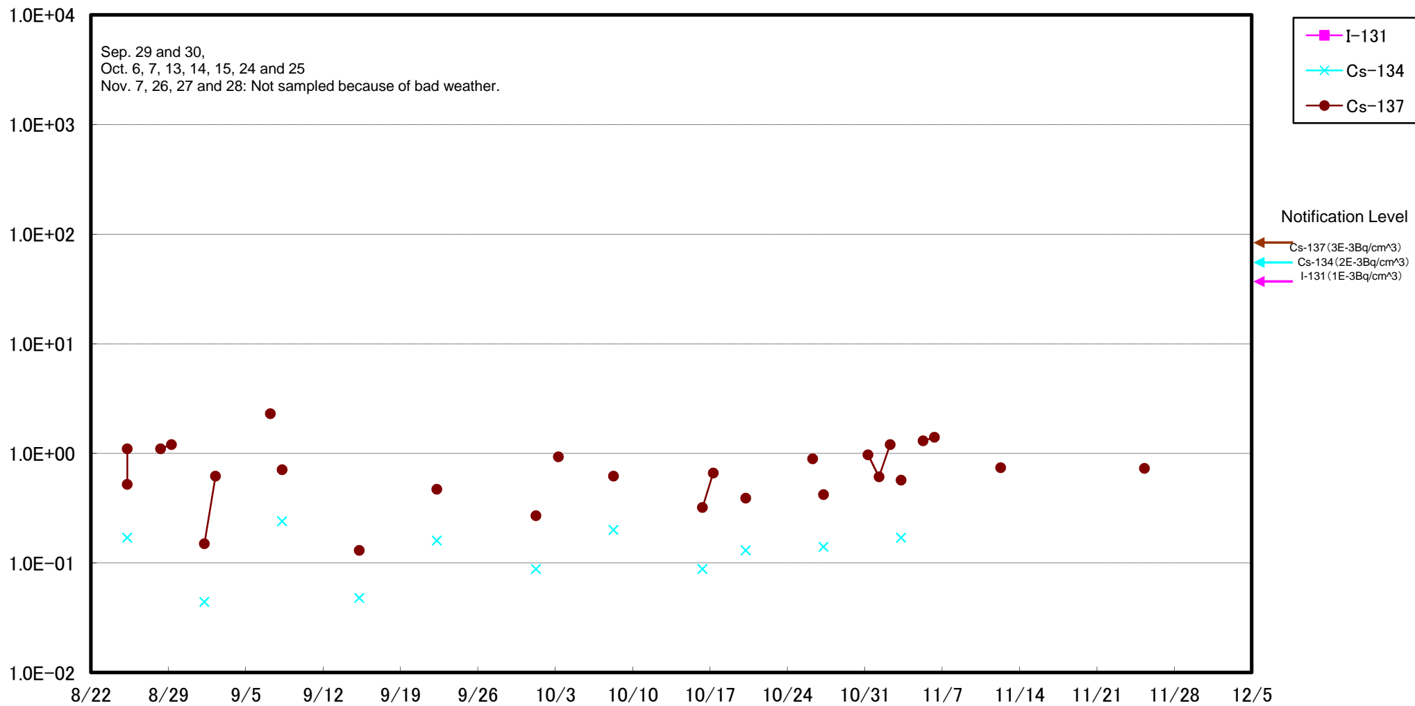
Radioactivity Density of the Seawater at 1F Units 5-6 North Discharge Channel (Bq/L)
