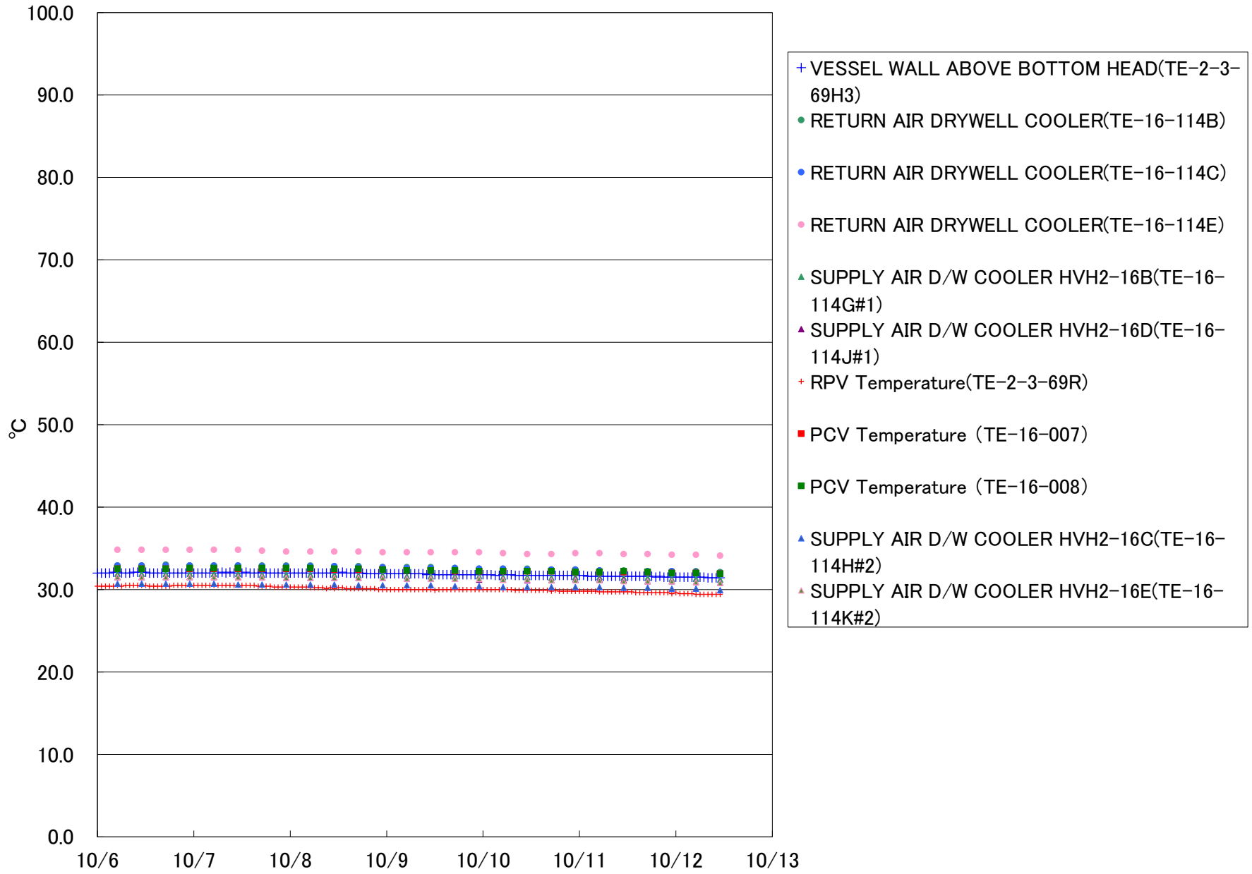
Fukushima Daiichi Nuclear Power Station Unit 2 Parameters of Temperature
