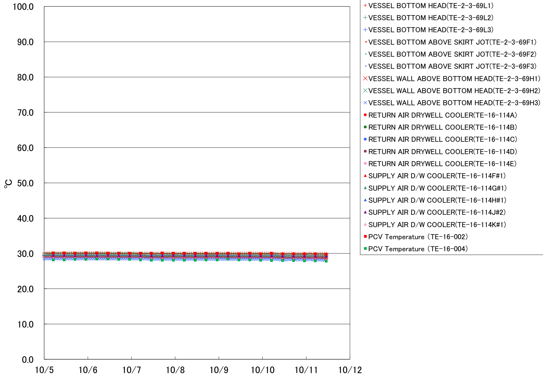
Fukushima Daiichi Nuclear Power Station Unit 3 Parameters of Temperature
