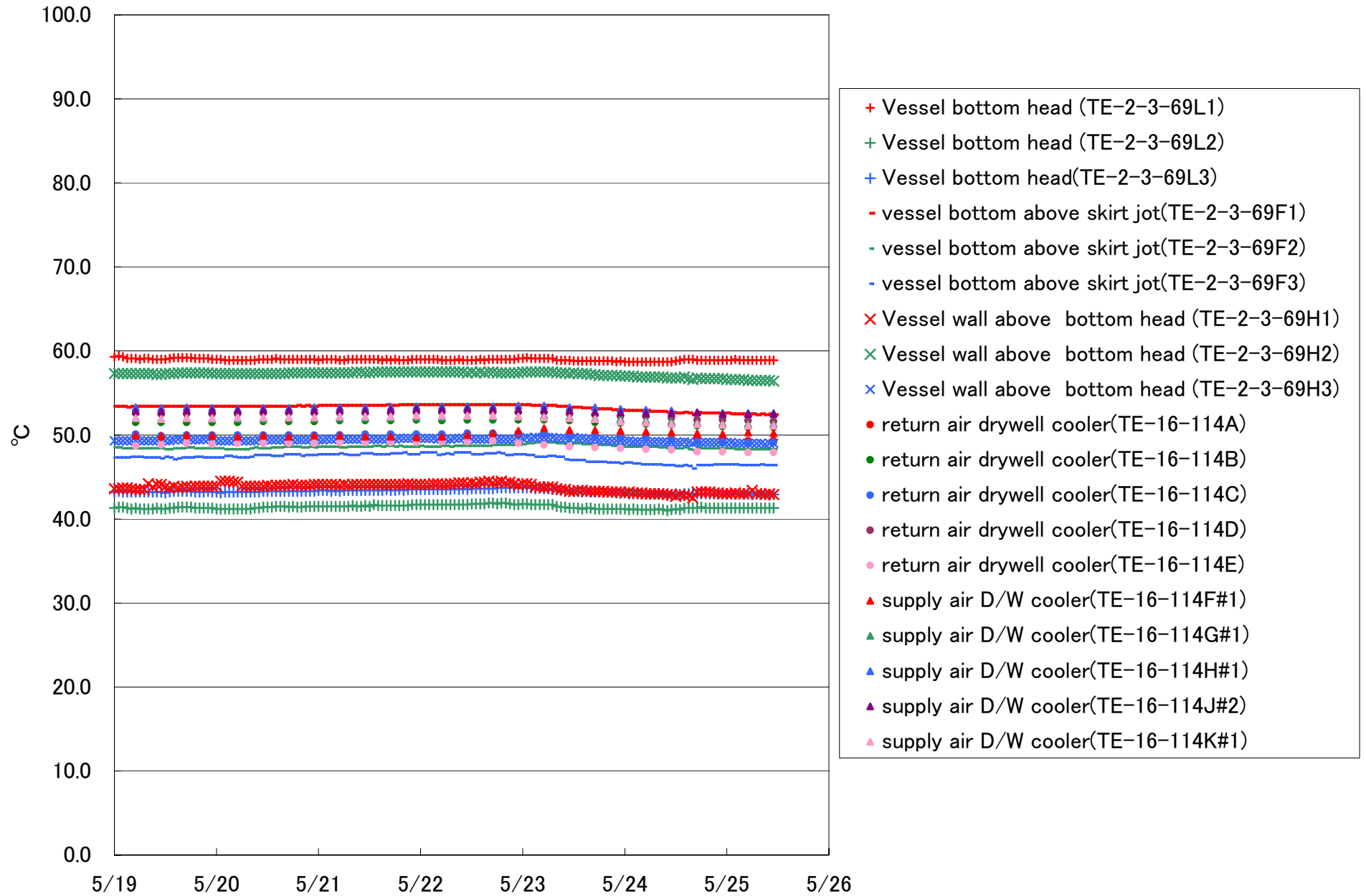
Fukushima Daiichi Nuclear Power Station Unit 3 Parameters of Temperature
