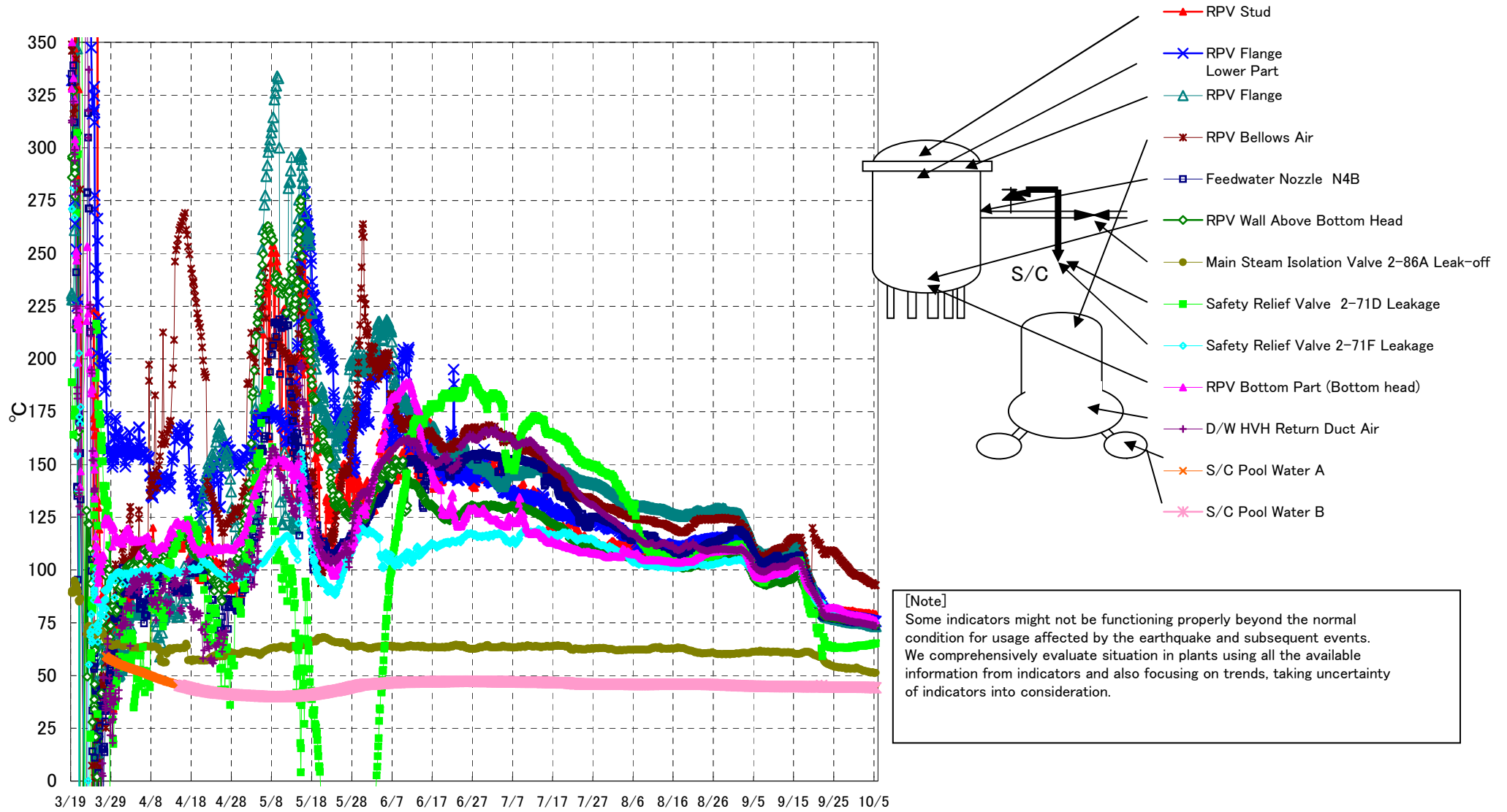
Fukushima Daiichi Nuclear Power Station Unit3 Parameters of Temperature (Typical Points)
