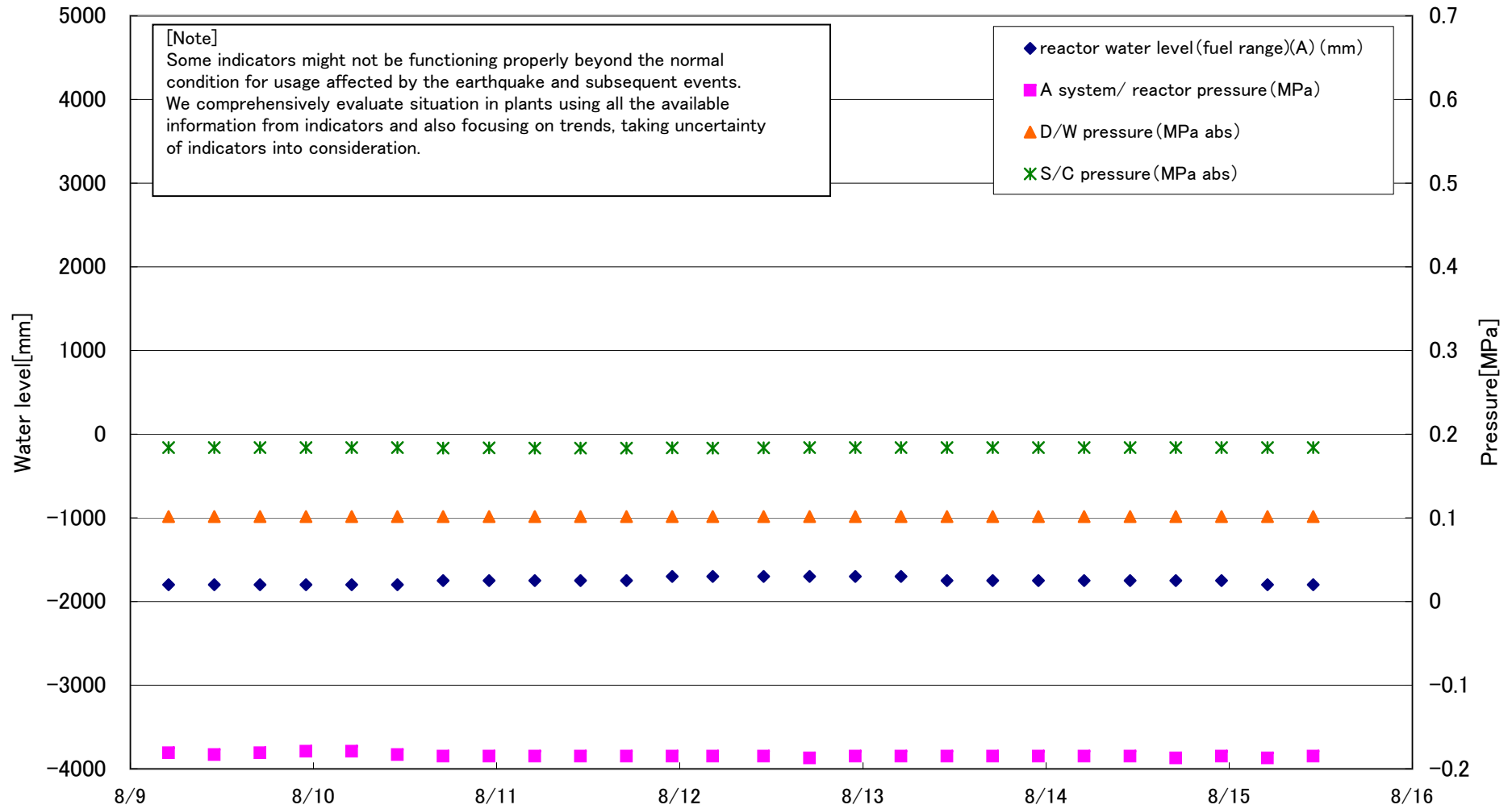
Fukushima Daiichi Nuclear Power Station Unit3 Parameters of Water level and Pressure
