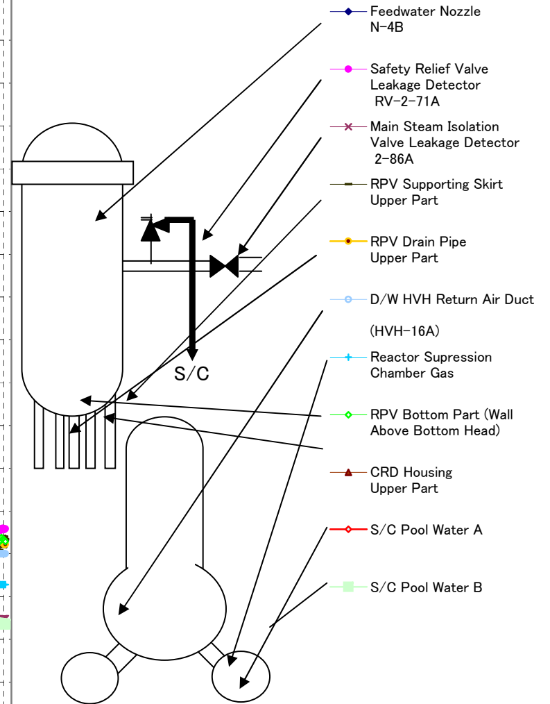
Fukushima Daiichi Nuclear Power Station Unit2 Parameters of Temperature (Typical Points)
