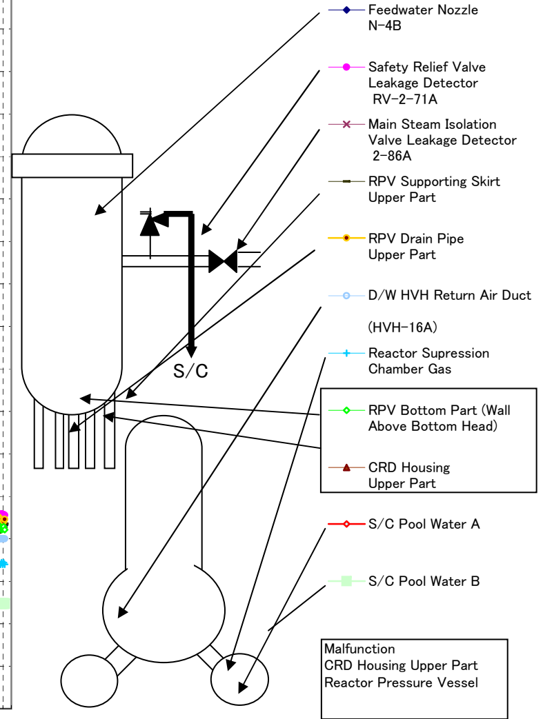
Fukushima Daiichi Nuclear Power Station Unit2 Parameters of Temperature (Typical Points)
