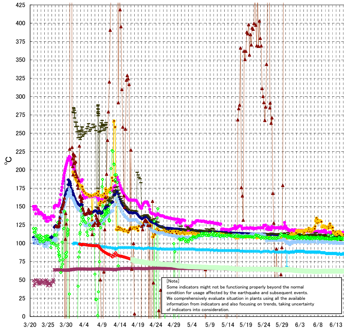
Fukushima Daiichi Nuclear Power Station Unit2 Parameters of Temperature (Typical Points)
