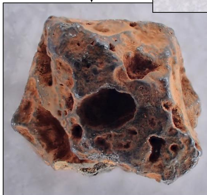
Enlarged photos of external appearance of fuel debris sample (taken from directly above)
