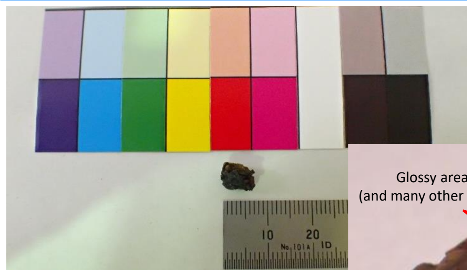
External appearance of fuel debris sample
