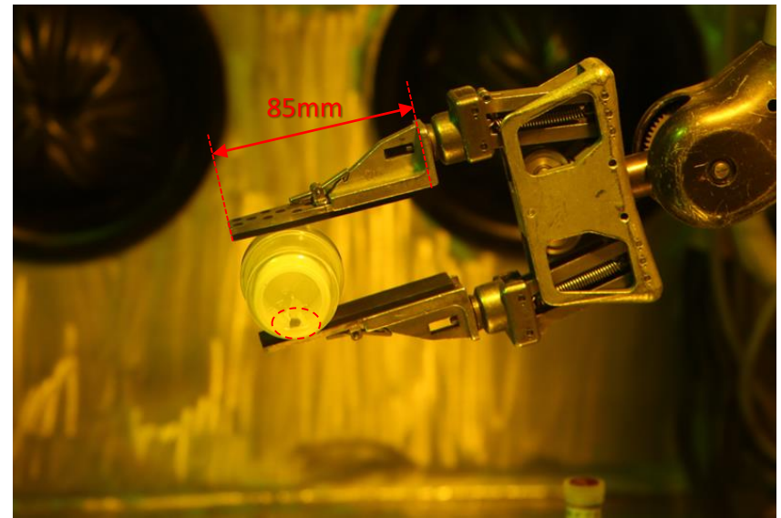
Fuel debris sample inside a specimen container
