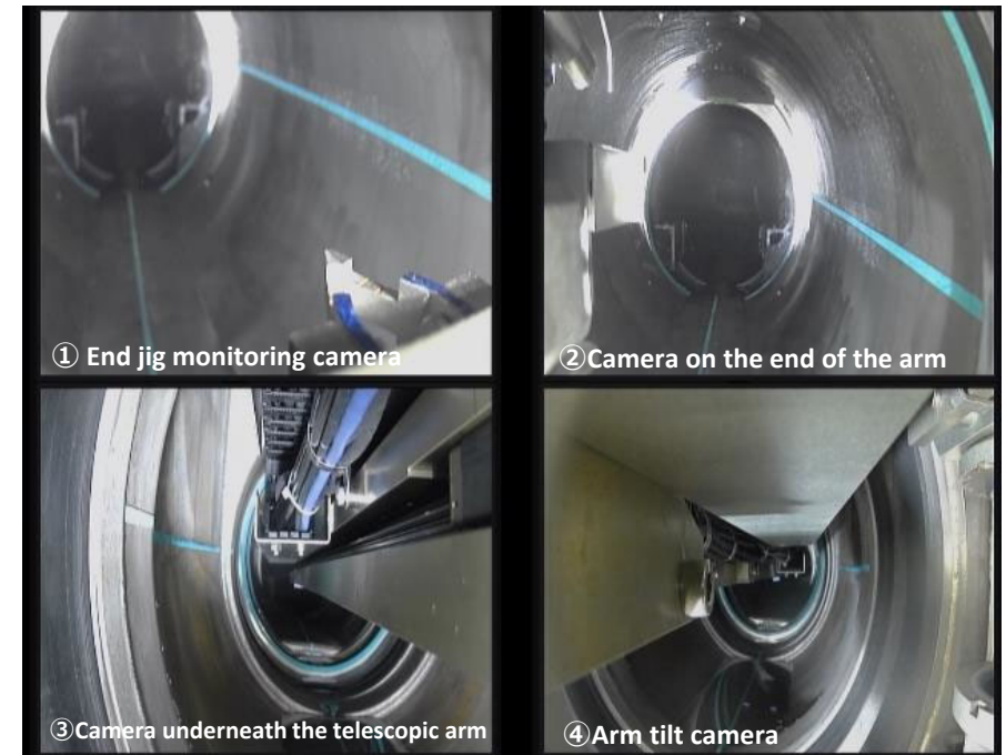
The end jig passing through the isolation valve
