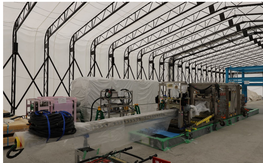
The entire view of the telescopic device (Guide pipe side)
