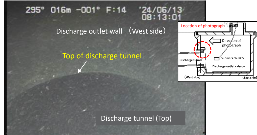
Discharge tunnel exit conditions (At connection with discharge outlet caisson)
