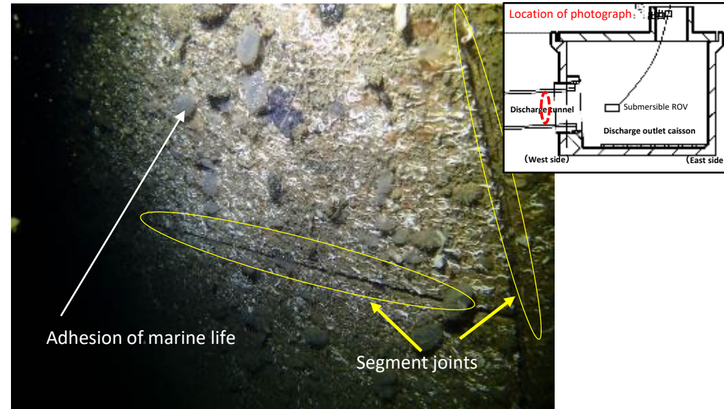
Conditions of wall near the discharge tunnel exit
