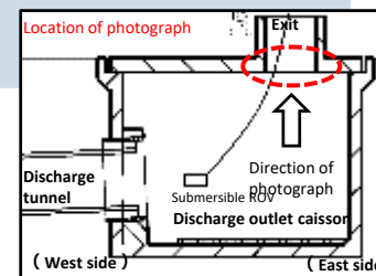
Discharge outlet caisson exit conditions
