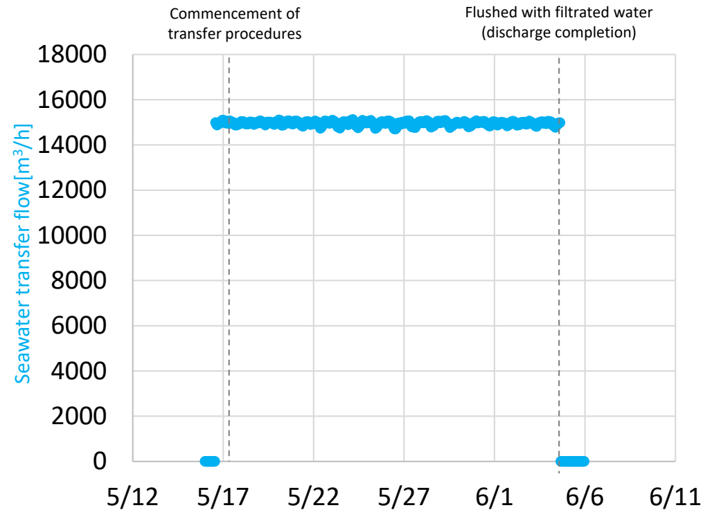
Seawater transfer flow
