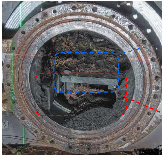
X-6 penetration (After the deposit removal work by low pressure water spray )
