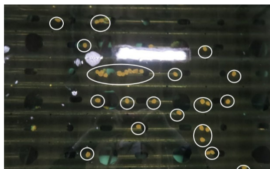
Feeding condition in regular seawater tank (Evening of February 13, 2023)
