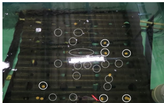
Leftover condition in regular seawater tank (Morning of February 14, 2023)
