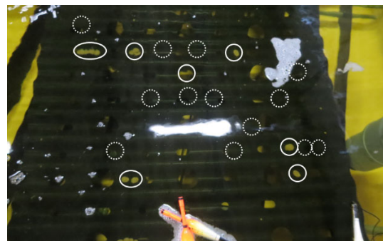
Leftover condition in ALPS treated water added tank (Morning of February 14, 2023)
