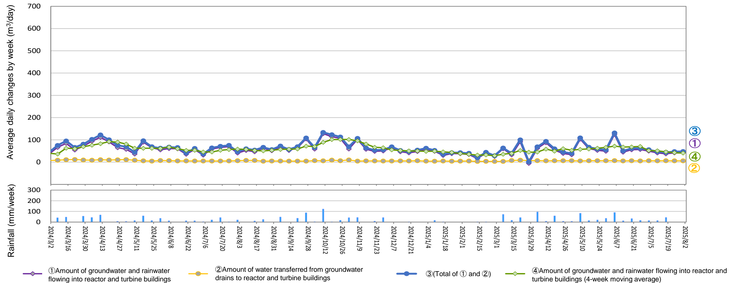
Amount of water transferred from groundwater drains to reactor and turbine buildings (From July 24, 2025 to July 30, 2025)
