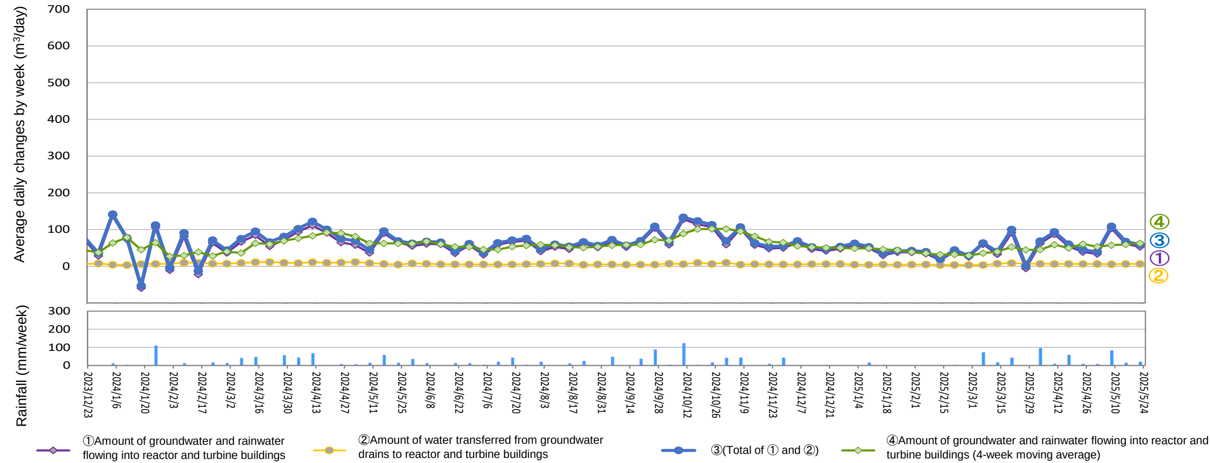
Amount of water transferred from groundwater drains to reactor and turbine buildings (From May 15, 2025 to May 21, 2025)
