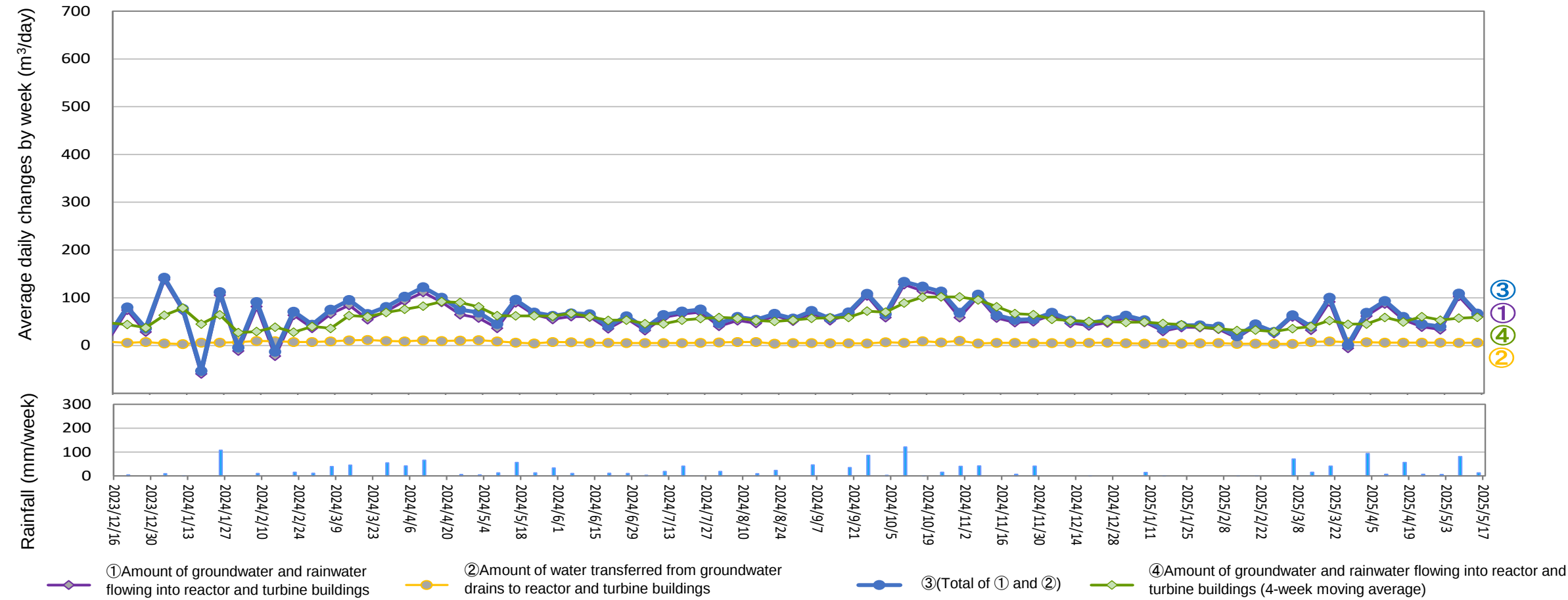
Amount of water transferred from groundwater drains to reactor and turbine buildings (From May 8, 2025 to May 14, 2025)
