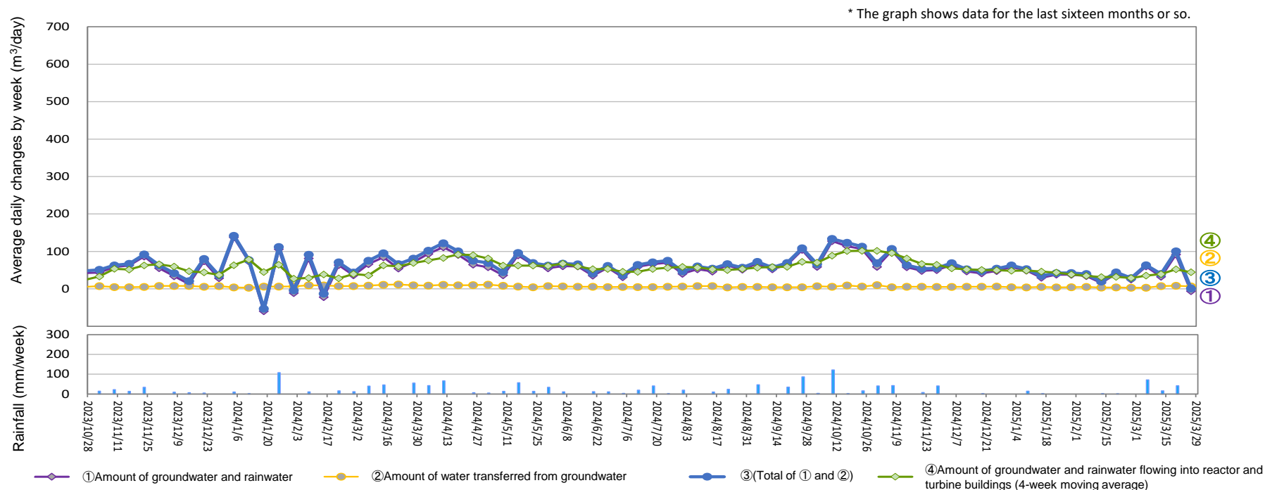
Amount of water transferred from groundwater drains to reactor and turbine buildings (From Mar 20, 2025 to Mar 26, 2025)
