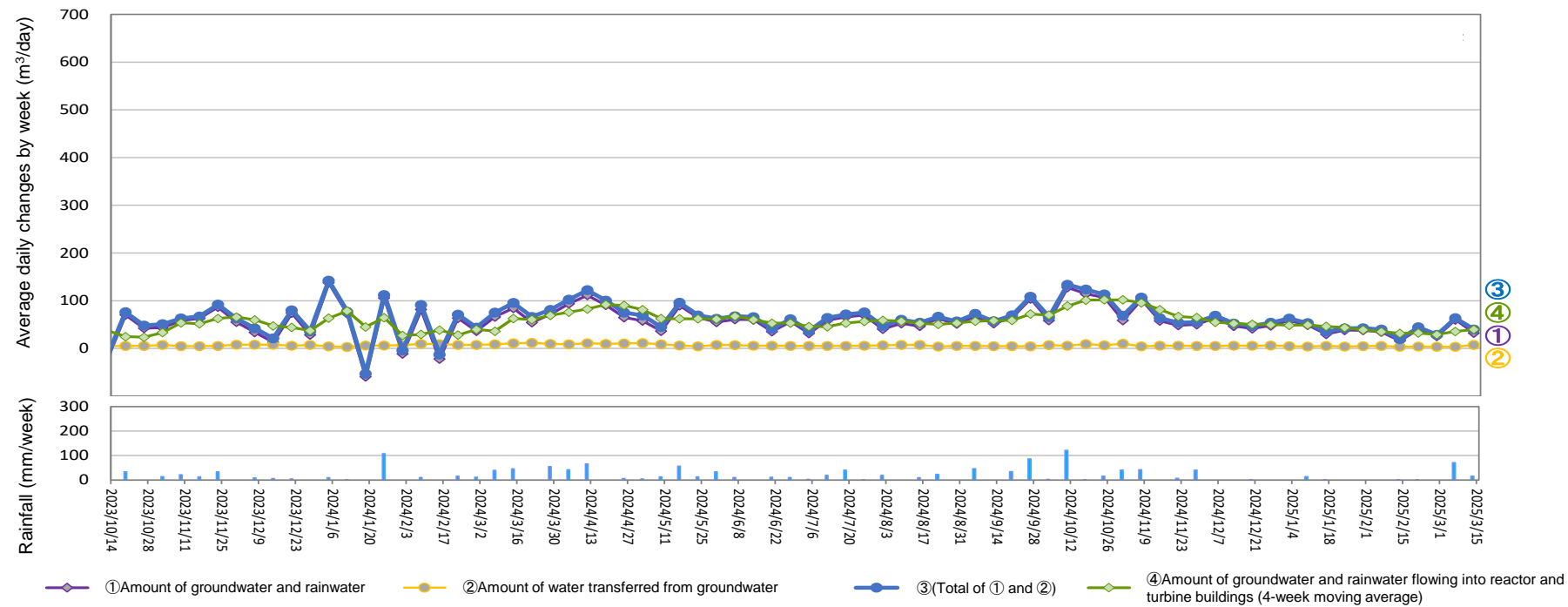
Amount of water transferred from groundwater drains to reactor and turbine buildings (From Mar 6, 2025 to Mar 12, 2025)
