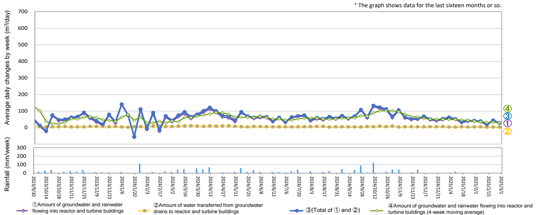
Amount of water transferred from groundwater drains to reactor and turbine buildings (From Feb 20, 2025 to Feb 26, 2025)
