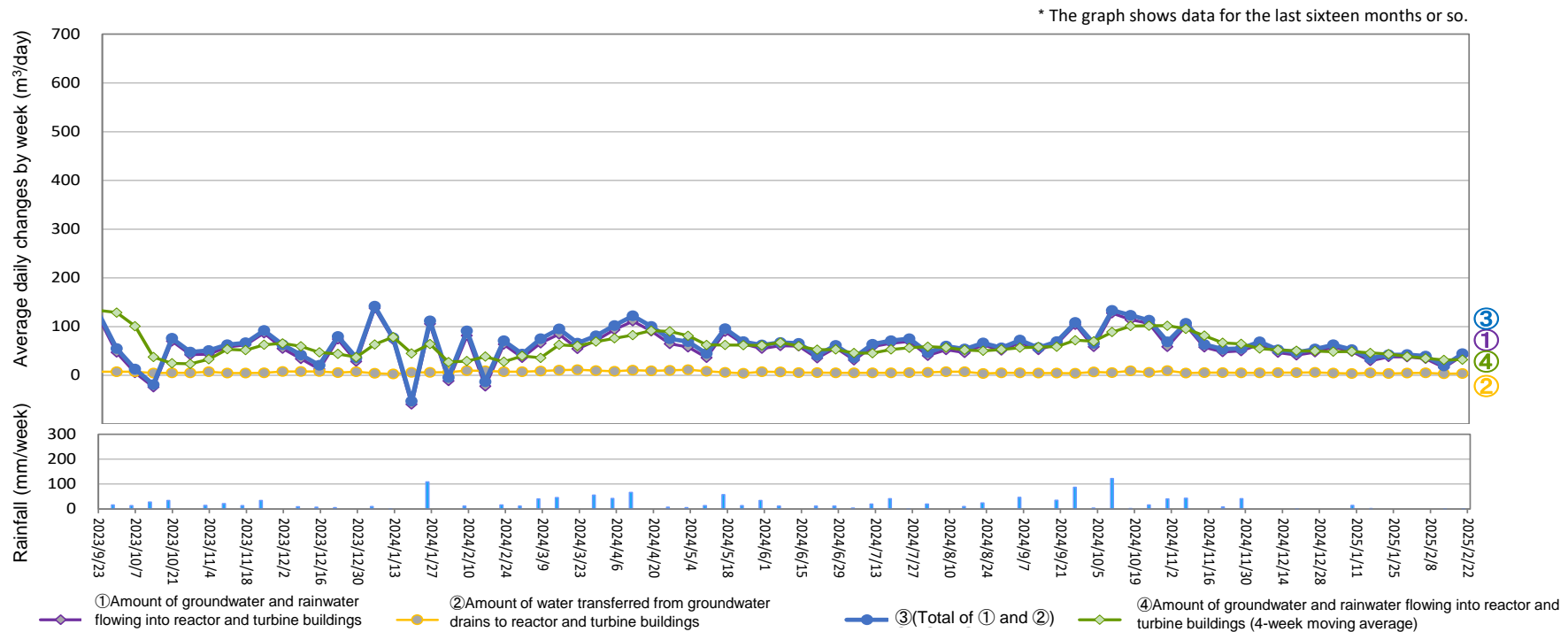
Amount of water transferred from groundwater drains to reactor and turbine buildings (From Feb 13, 2025 to Feb 19, 2025)
