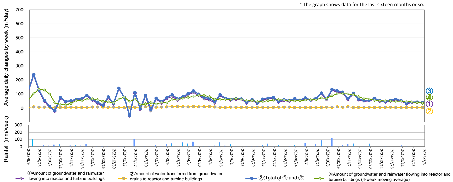
Amount of water transferred from groundwater drains to reactor and turbine buildings (From Jan 30, 2025 to Feb 5, 2025)
