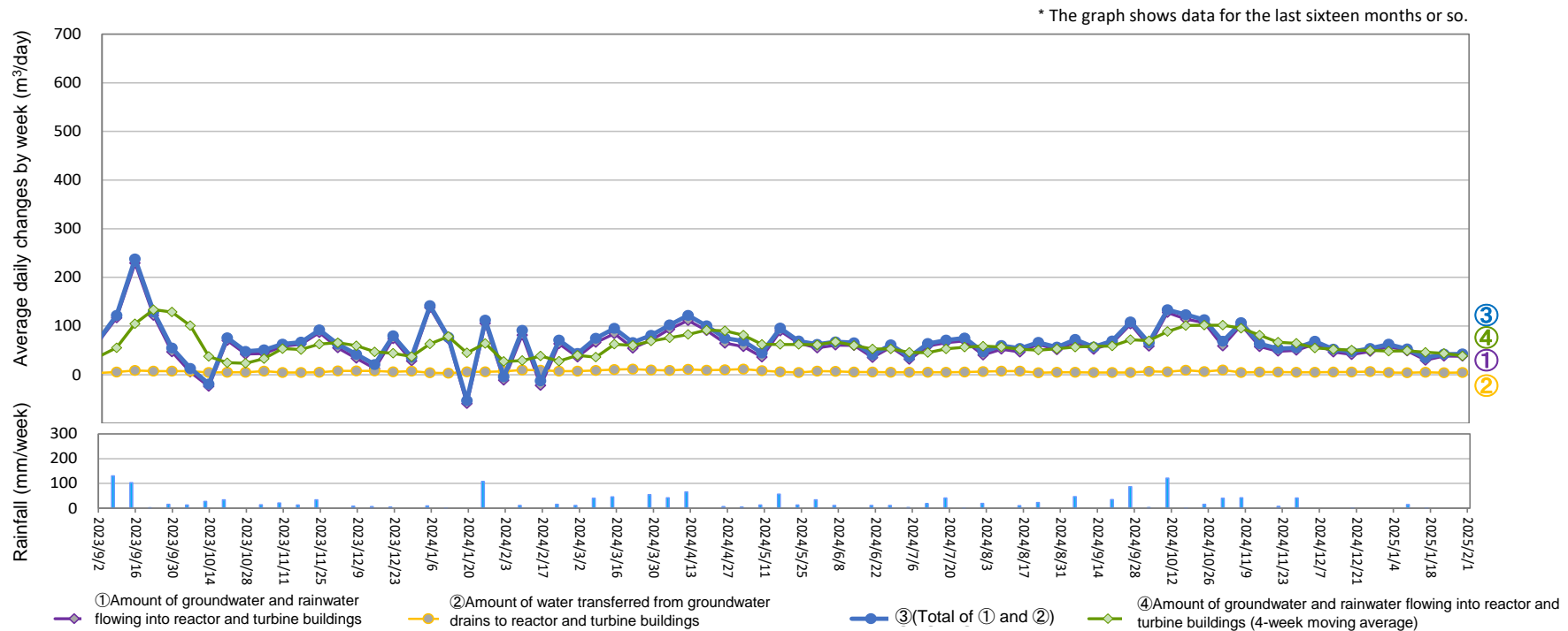
Amount of water transferred from groundwater drains to reactor and turbine buildings (From Jan 23, 2025 to Jan 29, 2025)
