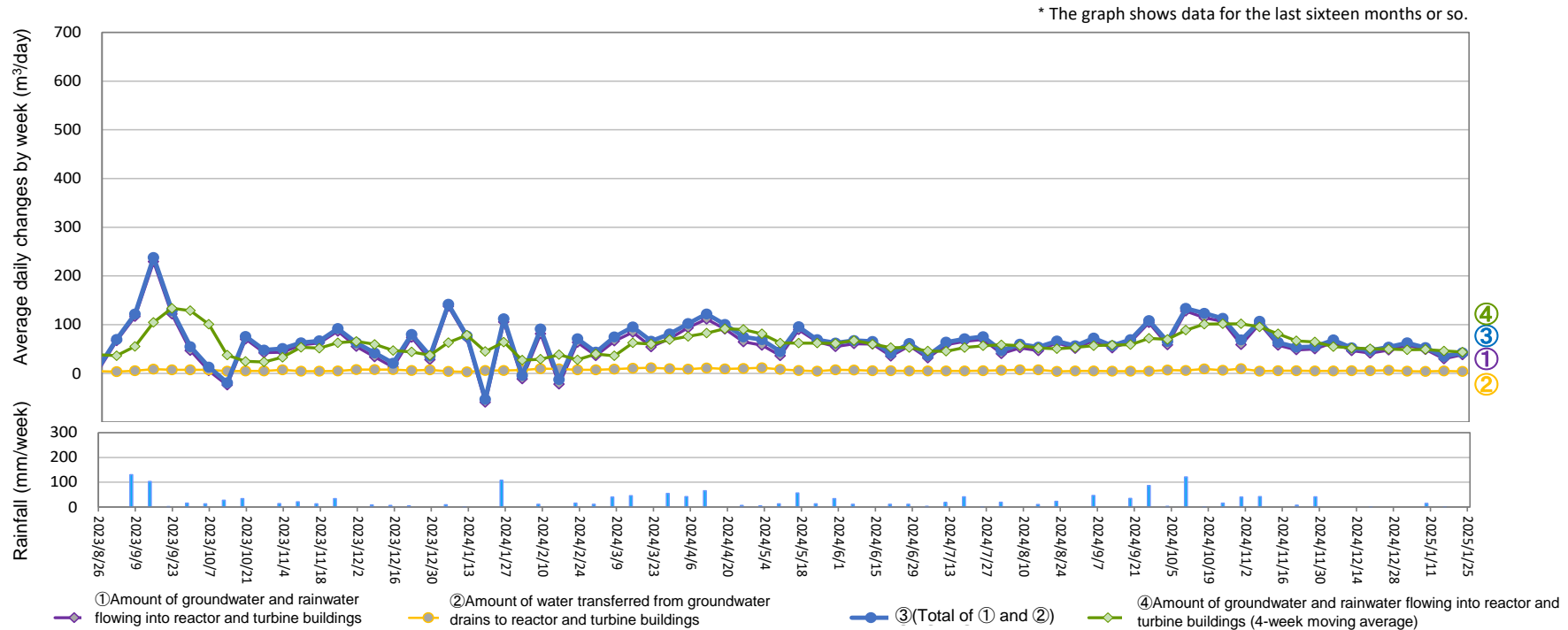
Amount of water transferred from groundwater drains to reactor and turbine buildings (From Jan 16, 2025 to Jan 22, 2025)
