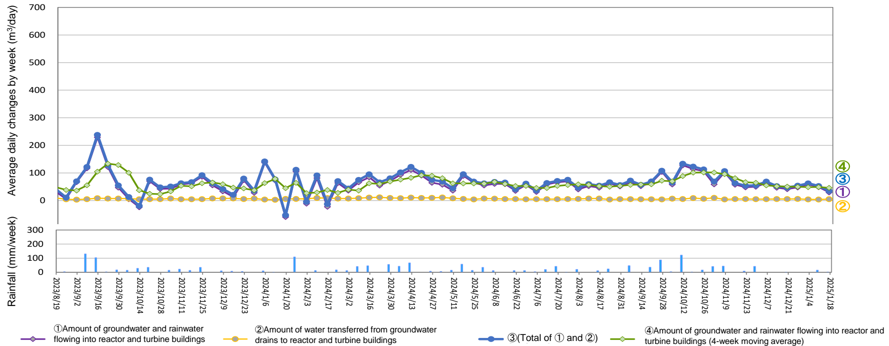
Amount of water transferred from groundwater drains to reactor and turbine buildings (From Jan 9, 2025 to Jan 15, 2025)
