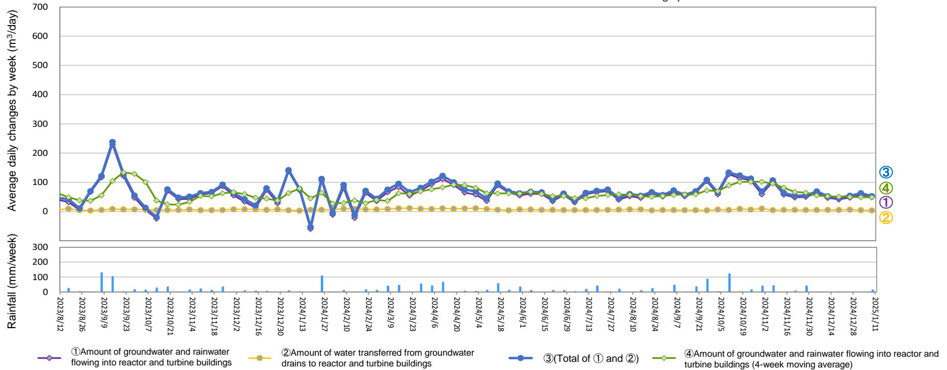
Amount of water transferred from groundwater drains to reactor and turbine buildings (From Jan 2, 2025 to Jan 8, 2025)
