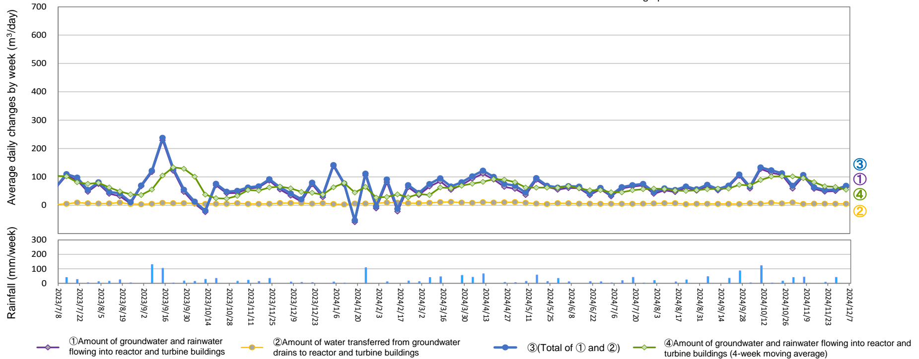
Amount of water transferred from groundwater drains to reactor and turbine buildings (From Nov 28, 2024 to Dec 4, 2024)
