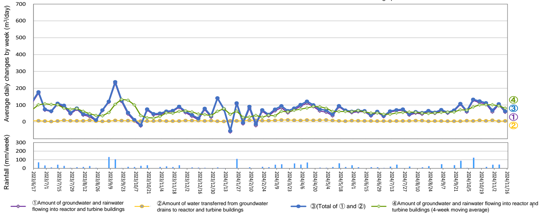
Amount of water transferred from groundwater drains to reactor and turbine buildings (From Nov 7, 2024 to Nov 13, 2024)
