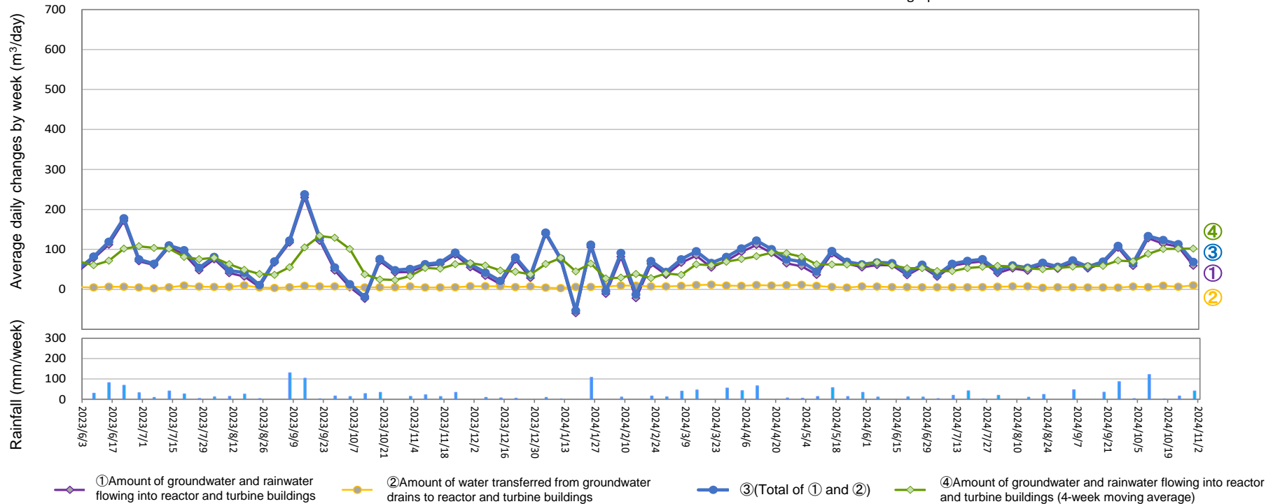
Amount of water transferred from groundwater drains to reactor and turbine buildings (From Oct 24, 2024 to Oct 30, 2024)
