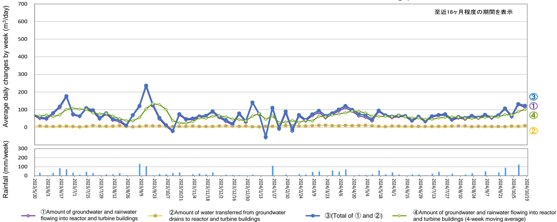
Amount of water transferred from groundwater drains to reactor and turbine buildings (From Oct 10, 2024 to Oct 16, 2024)
