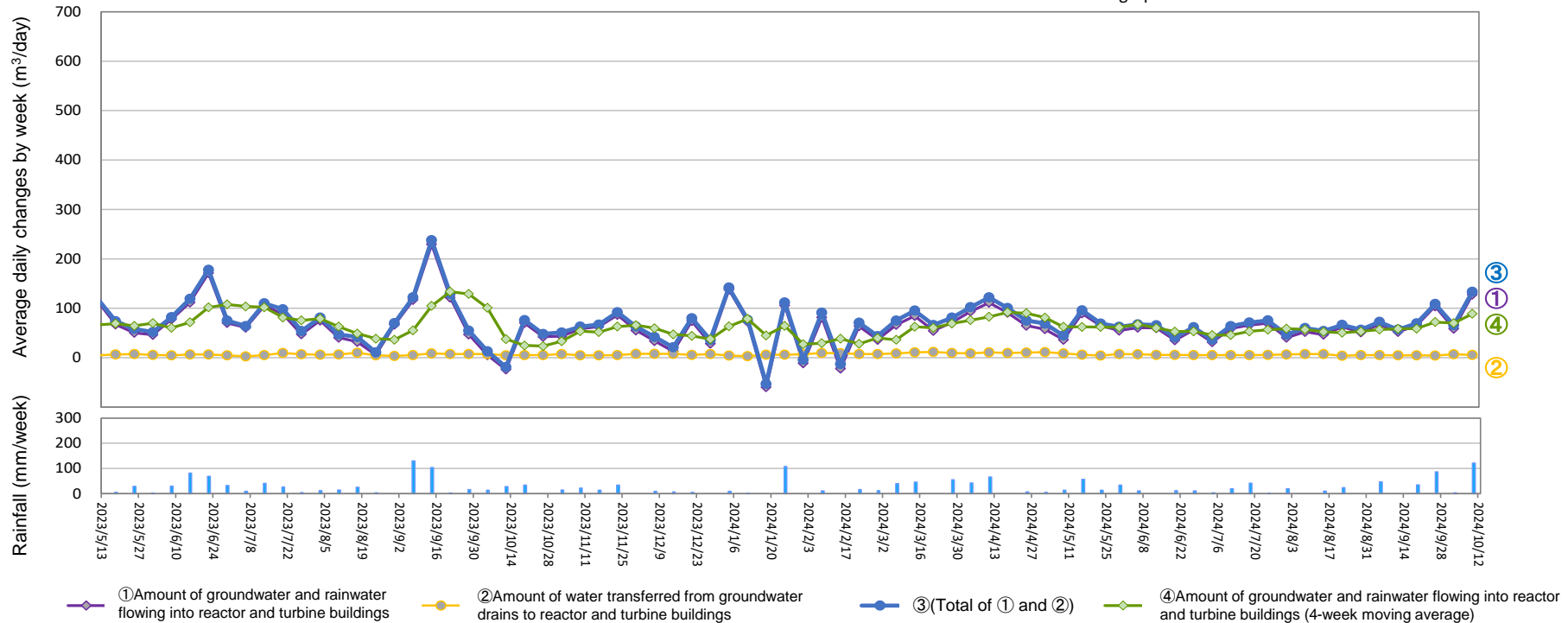
Amount of water transferred from groundwater drains to reactor and turbine buildings (From Oct 3, 2024 to Oct 9, 2024)
