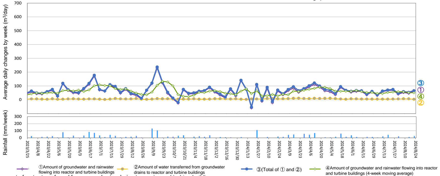
Amount of water transferred from groundwater drains to reactor and turbine buildings (From Aug 15, 2024 to Aug 21, 2024)
