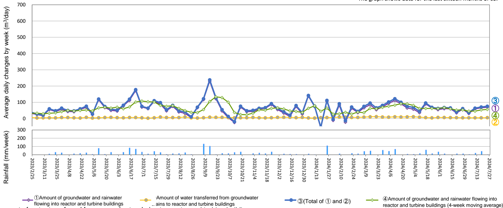
Amount of water transferred from groundwater drains to reactor and turbine buildings (From July 18, 2024 to July 24, 2024)
