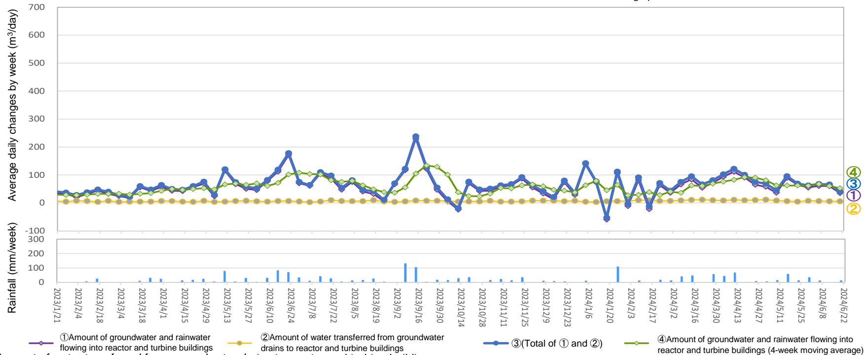
Amount of water transferred from groundwater drains to reactor and turbine buildings (From June 13, 2024 to June 19, 2024)
