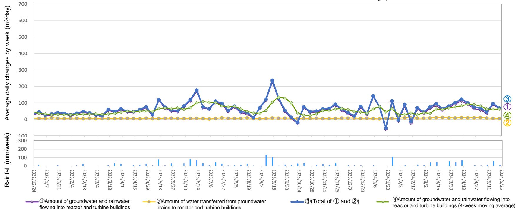
Amount of water transferred from groundwater drains to reactor and turbine buildings (From May 16, 2024 to May 22, 2024)
