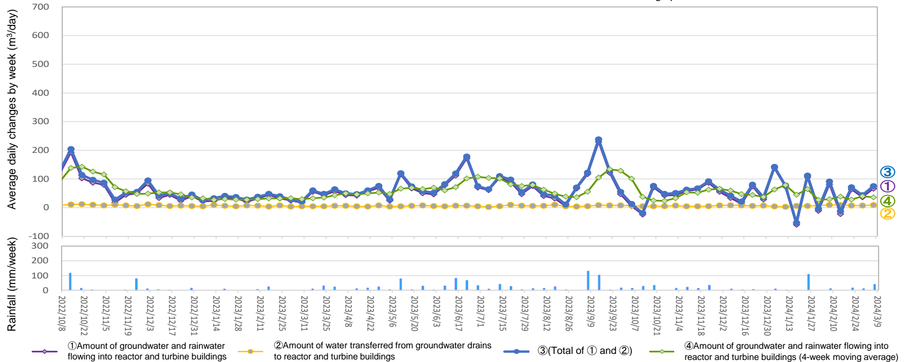
Amount of water transferred from groundwater drains to reactor and turbine buildings (From February 29, 2024 to March 6, 2024)
