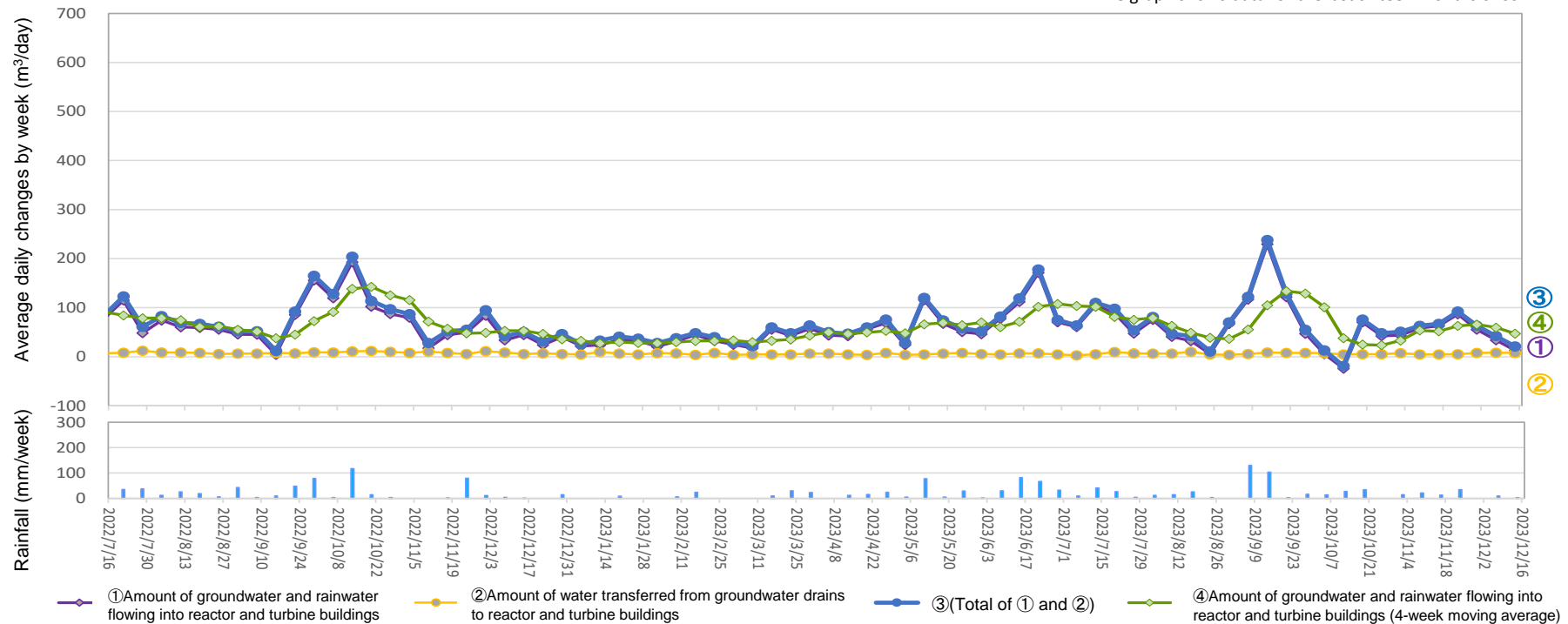
Amount of water transferred from groundwater drains to reactor and turbine buildings (From December 7, 2023 to December 13, 2023)
