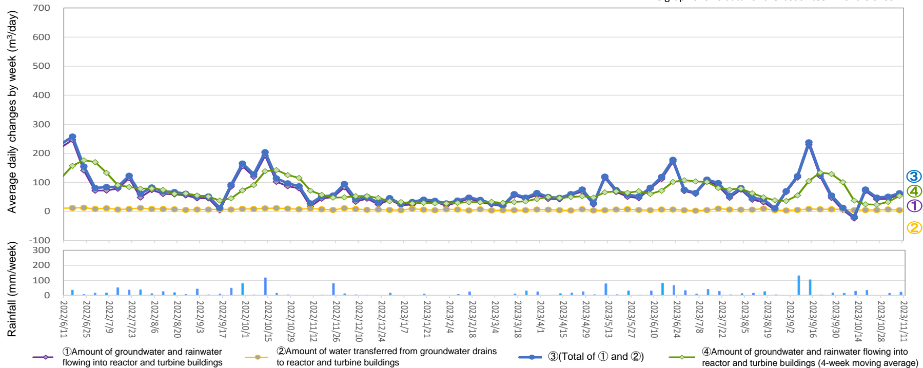
Amount of water transferred from groundwater drains to reactor and turbine buildings (From November 2, 2023 to November 8, 2023)
