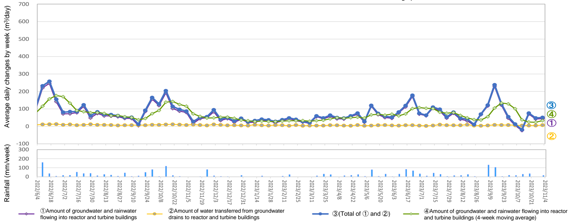
Amount of water transferred from groundwater drains to reactor and turbine buildings (From October 26, 2023 to November 1, 2023)
