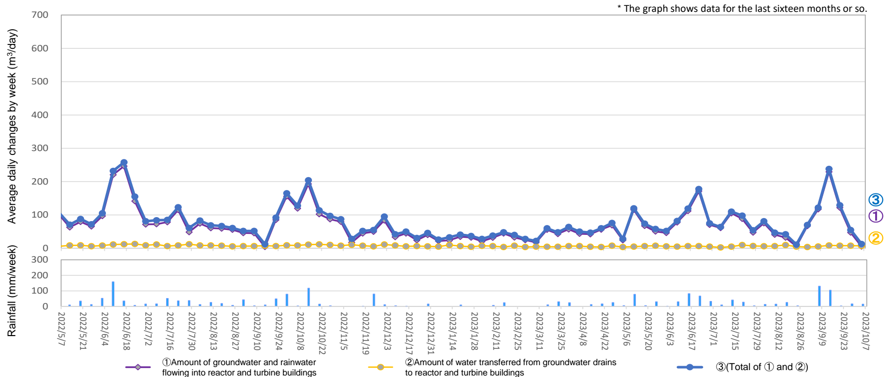
Amount of water transferred from groundwater drains to reactor and turbine buildings (From September 28, 2023 to October 4, 2023)
