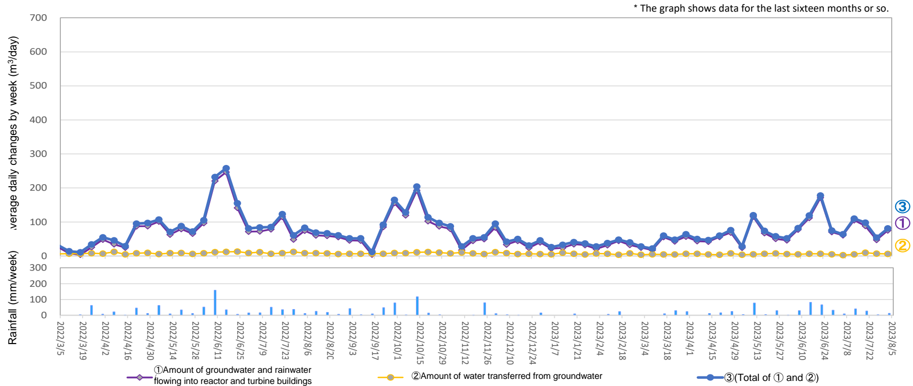
Amount of water transferred from groundwater drains to reactor and turbine buildings (From July 27, 2023 to August 2, 2023)
