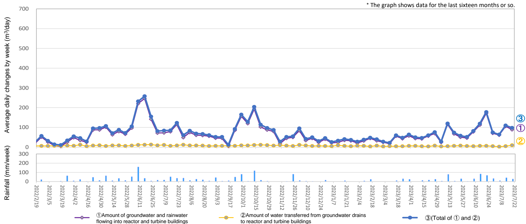
Amount of water transferred from groundwater drains to reactor and turbine buildings (From July 13, 2023 to July 19, 2023)
