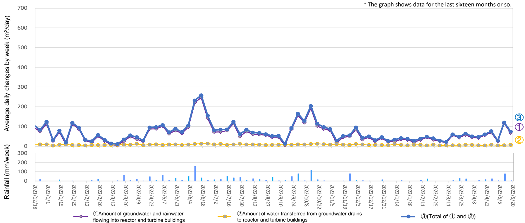
Amount of water transferred from groundwater drains to reactor and turbine buildings (From May 11, 2023 to May 17, 2023)
