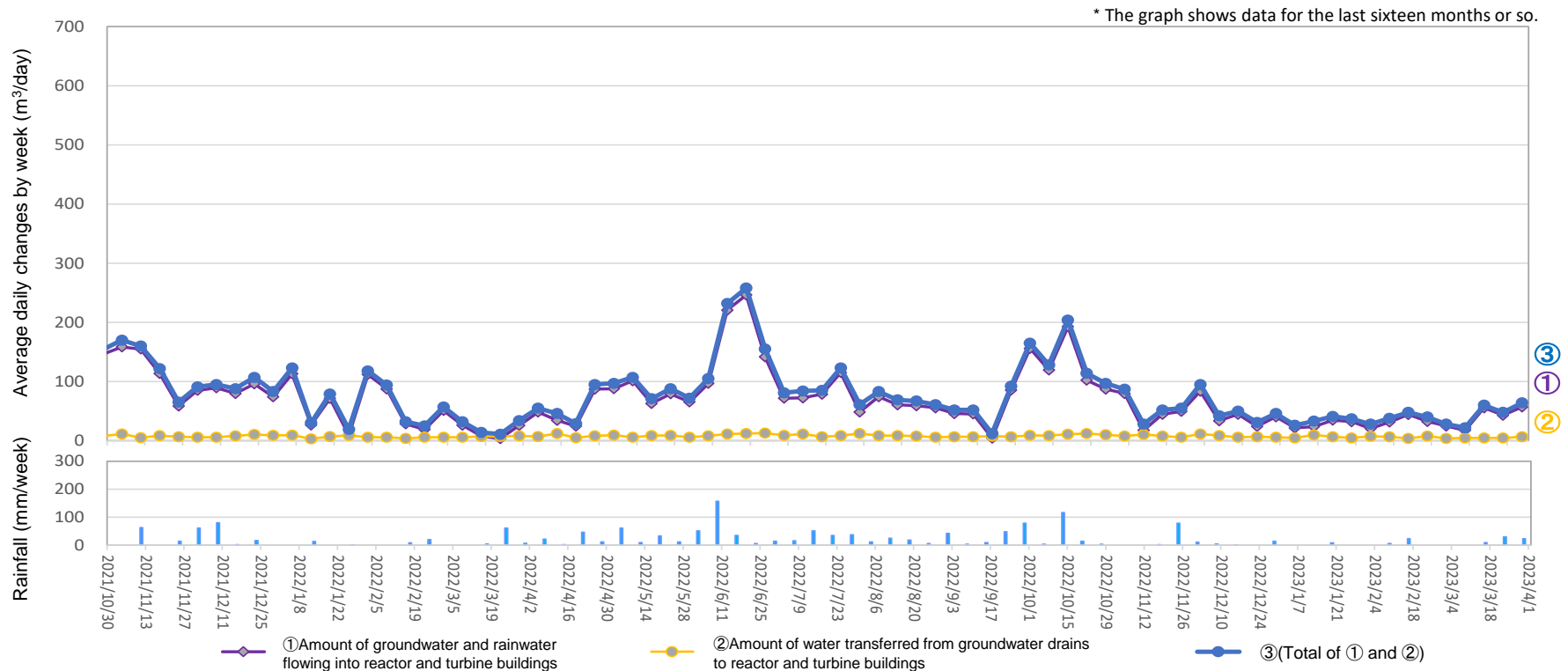
Amount of water transferred from groundwater drains to reactor and turbine buildings (From March 23, 2023 to March 29, 2023)
