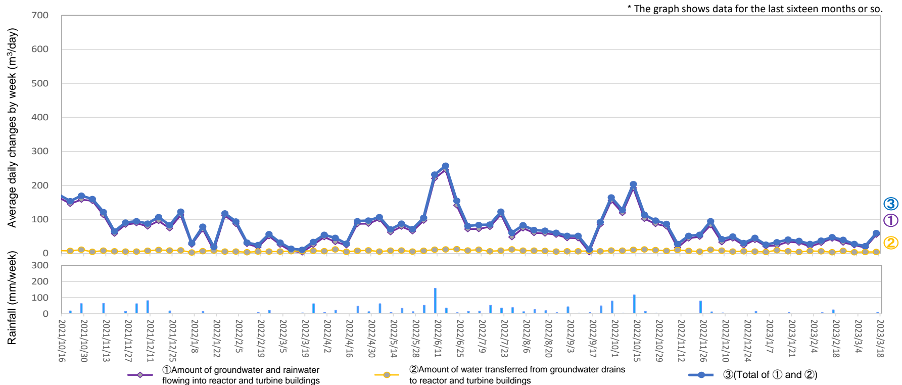
Amount of water transferred from groundwater drains to reactor and turbine buildings (From March 9, 2023 to March 15, 2023)
