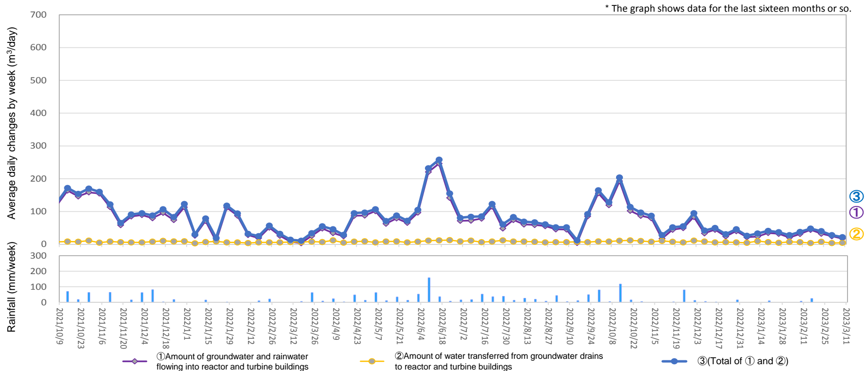
Amount of water transferred from groundwater drains to reactor and turbine buildings (From March 2, 2023 to March 8, 2023)
