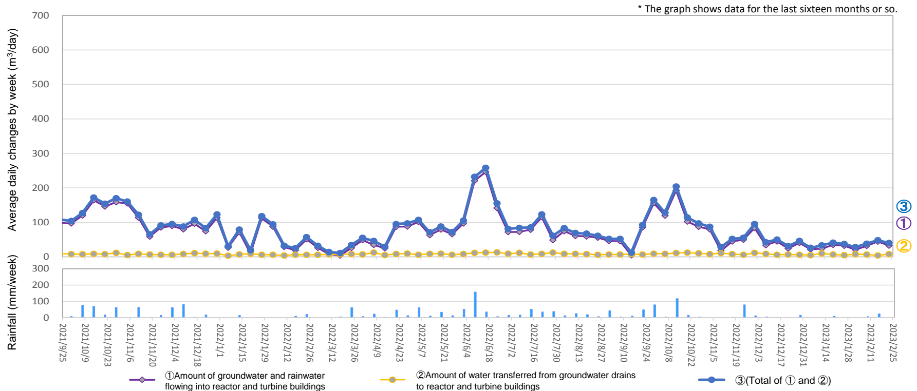
Amount of water transferred from groundwater drains to reactor and turbine buildings (From February 16, 2023 to February 22, 2023)
