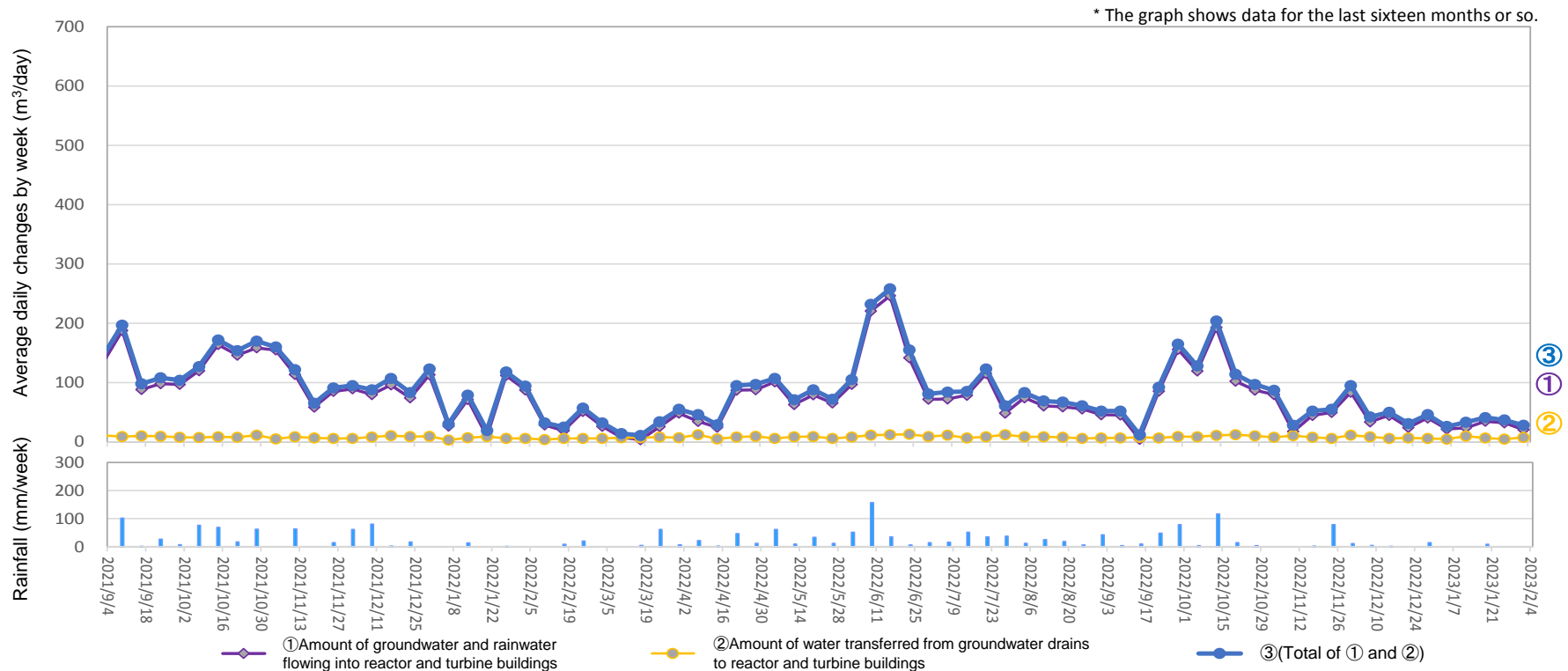
Amount of water transferred from groundwater drains to reactor and turbine buildings (From January 26, 2023 to February 1, 2023)
