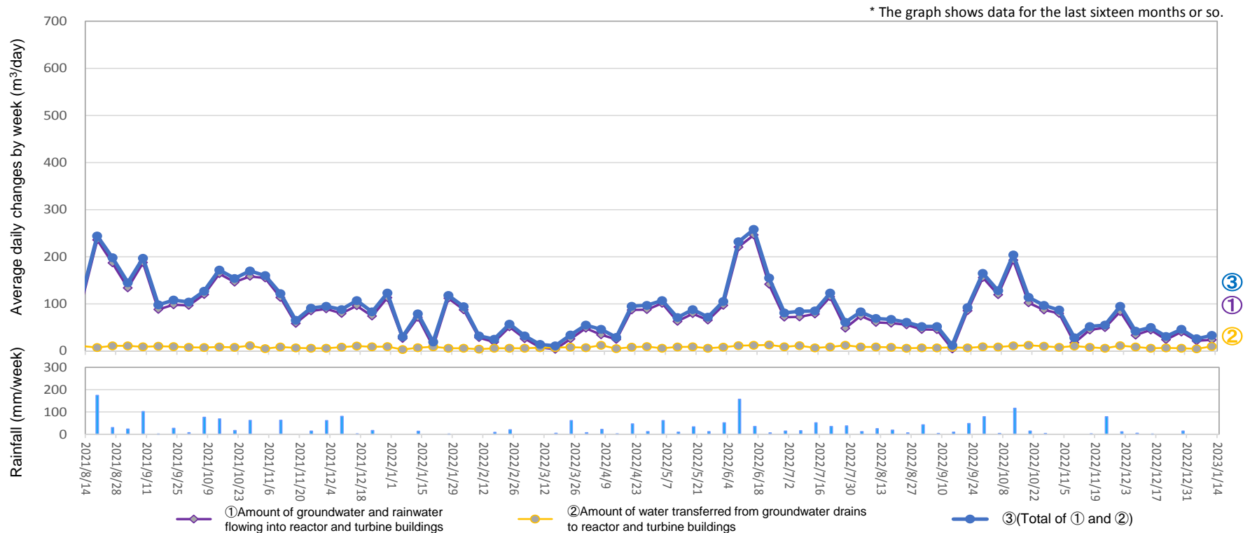
Amount of water transferred from groundwater drains to reactor and turbine buildings (From January 5, 2023 to January 11, 2023)
