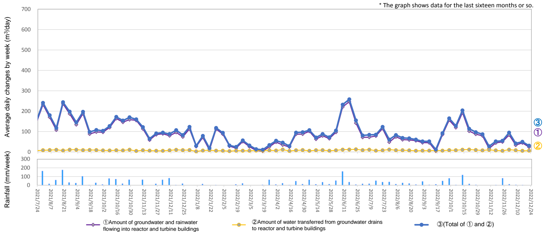
Amount of water transferred from groundwater drains to reactor and turbine buildings (From December 15, 2022 to December 21, 2022)
